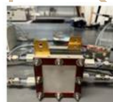
Ammonia fuel cell
